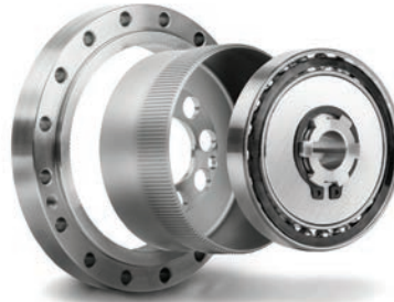
Component WPC-□-□-CR WPC-□-□-CD
